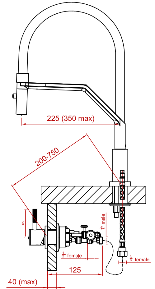
Horizontal control valve example
