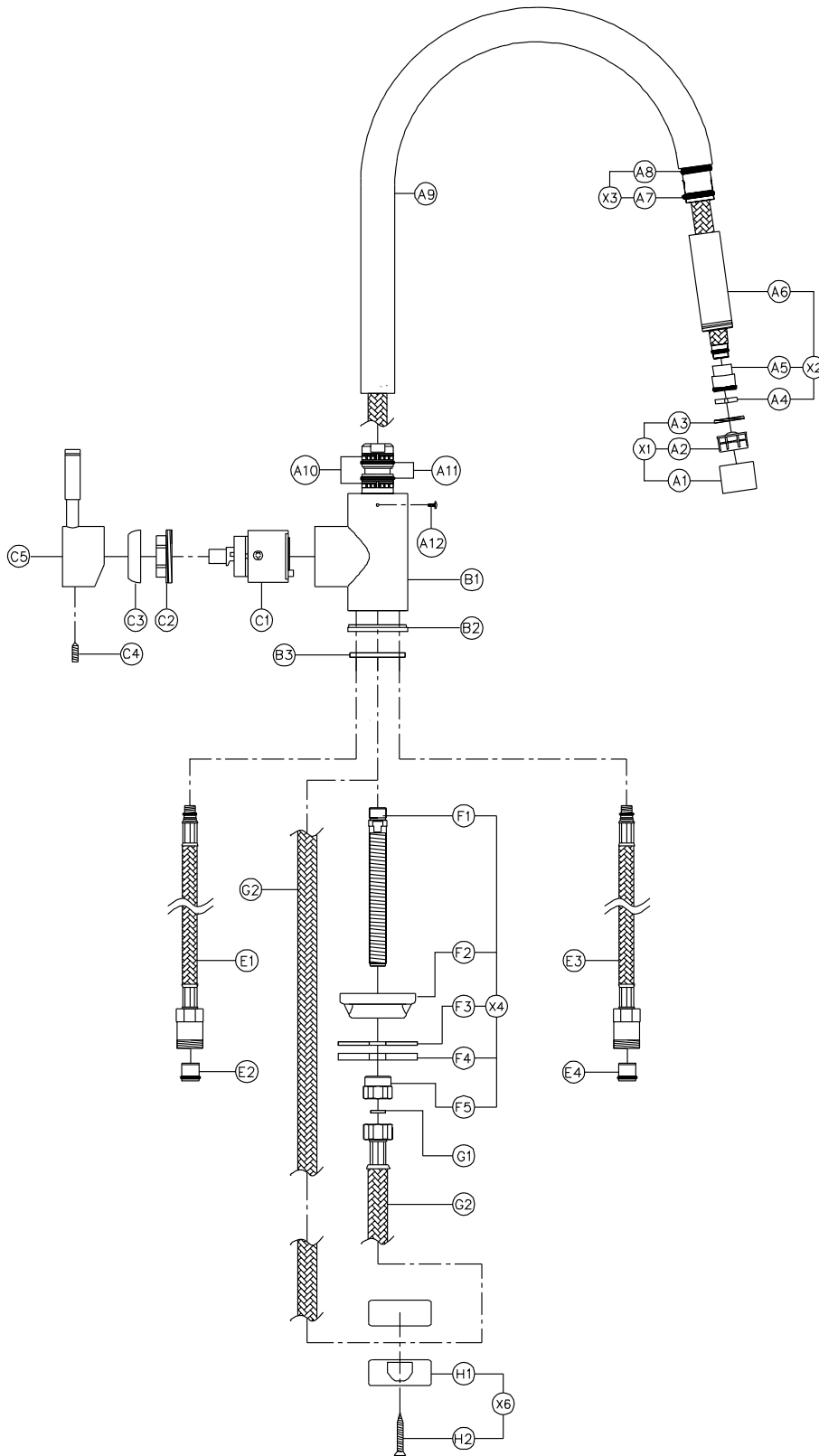
TRE1SLPO - Aquatrend single lever pull out service drawing v1
