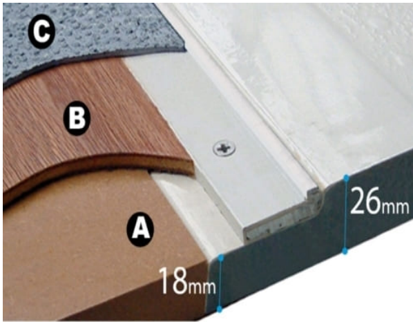
A - Floorboard or concrete floor B - ¼" plywood C - 2mm vinyl sheet flooring
