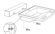
Mounting R1201
