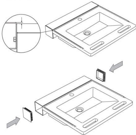
Mounting R1201
