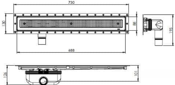
Side Outlet
