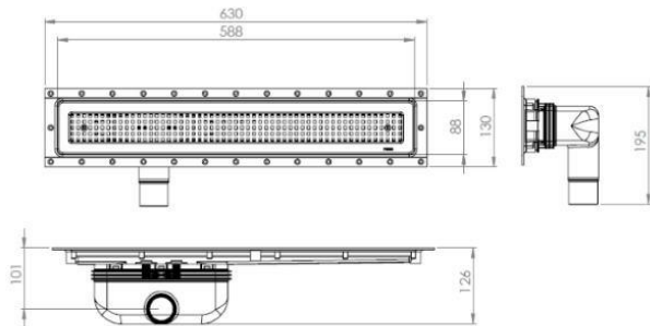
Side Outlet
