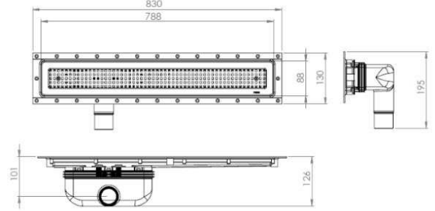
Side Outlet
