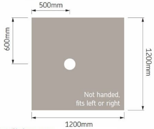
AKW Tuff Form® Former only: 21018
