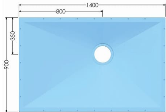
AKW Tuff Form® Former only: 21028
