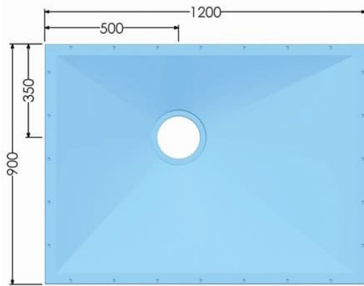
AKW Tuff Form® Former only: 21015
