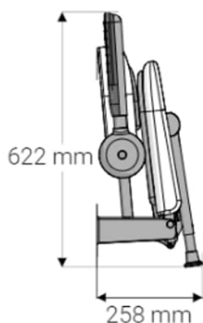
Folded Dimensions
