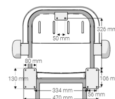
Mounting Hole Dimensions
