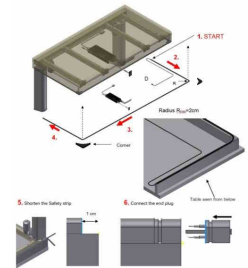
Mounting the safety stop strip - See PDF Installation Instructions
