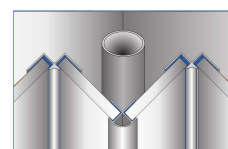
Ensure all trims are fixed with Showerwall adhesive and the trim recesses are filled with Showerwall sealant prior to installing the panel sections.
