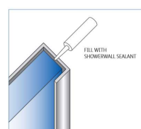
End trims 2450mm. Finishing end cap for square cut edge panel. Seal with Showerwall sealant.
