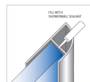
Quadrant trims 2450mm. Finishing end cap for square cut edge panel. Seal with Showerwall sealant.
