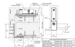
Royde & Tucker H131-100 HI-LOAD pivot set
